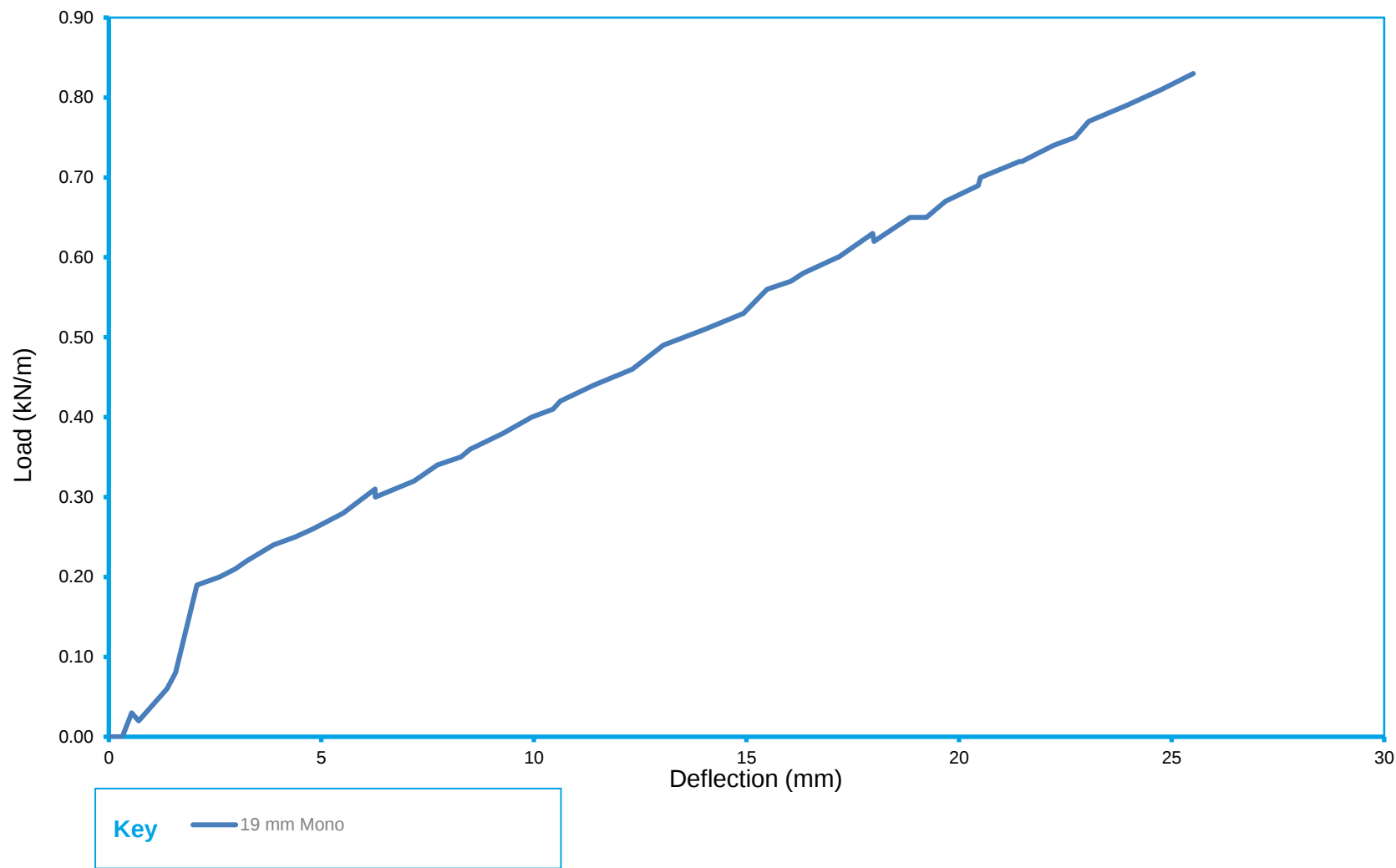
Chart 3 - Load Versus Deflection Curve for OnLevel TL-6621 Side Mounted Balustrade System Horizontal Line Load
