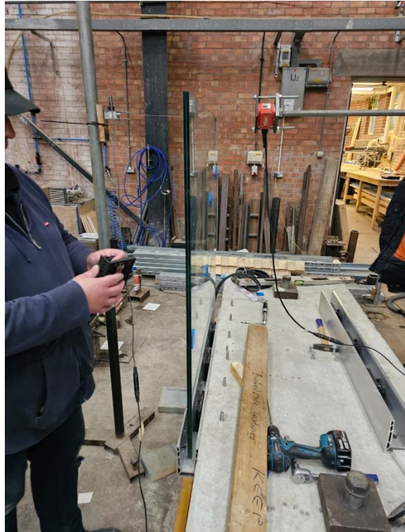
Plate 1 – Generic Test Arrangement
