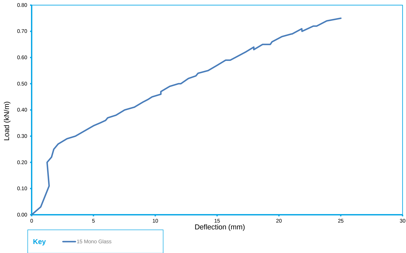
Chart 2 - Load Versus Deflection Curve for OnLevel TL-6621 Side Mounted Balustrade System Horizontal Line Load
