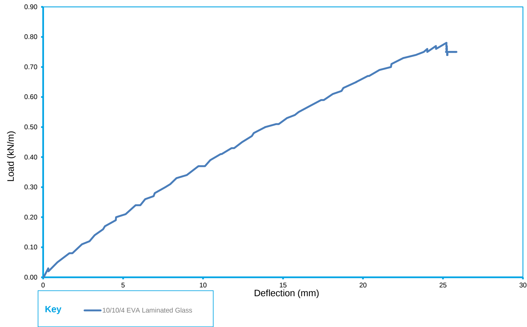
Chart 4 - Load Versus Deflection Curve for OnLevel TL-6621 Side Mounted Balustrade System Horizontal Line Load
