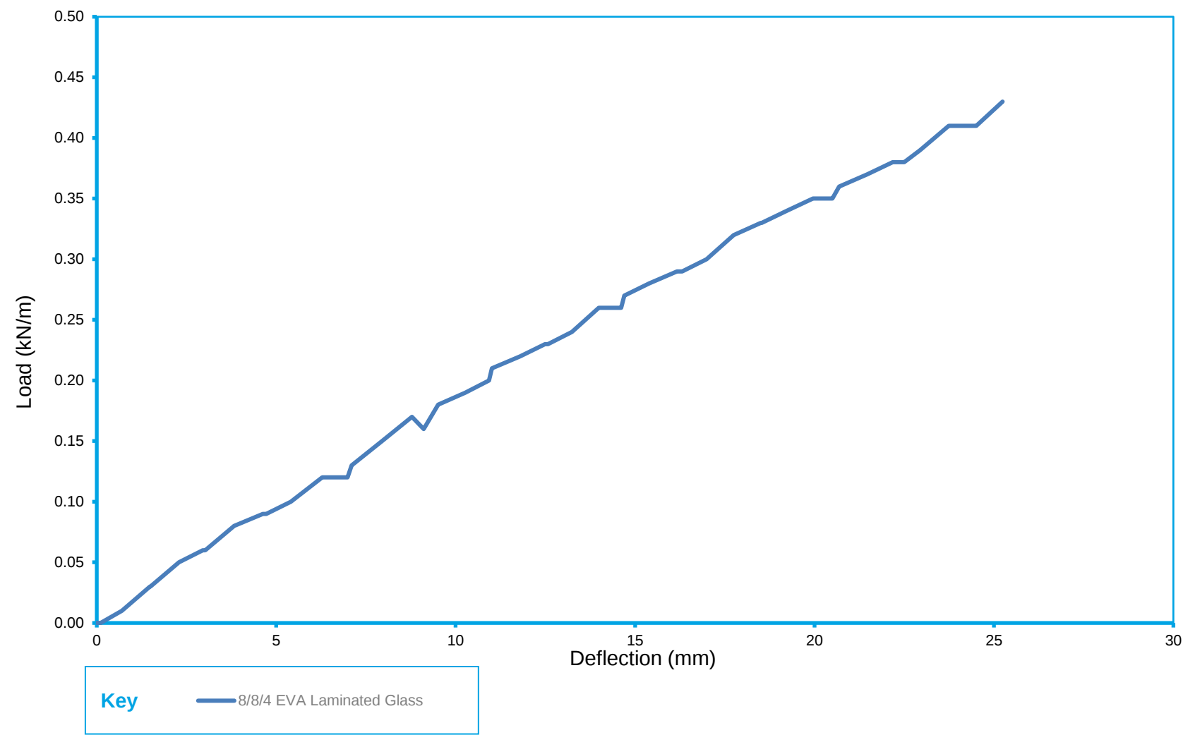
Chart 1 - Load Versus Deflection Curve for OnLevel TL-6621 Side Mounted Balustrade System Horizontal Line Load
