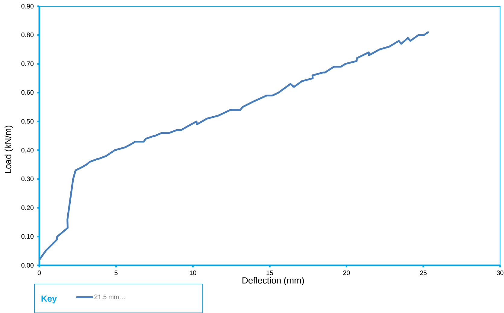
Chart 5 - Load Versus Deflection Curve for OnLevel TL-6621 Side Mounted Balustrade System Horizontal Line Load
