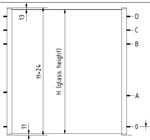
Skyforce-SLIM Top mount screw position overview
